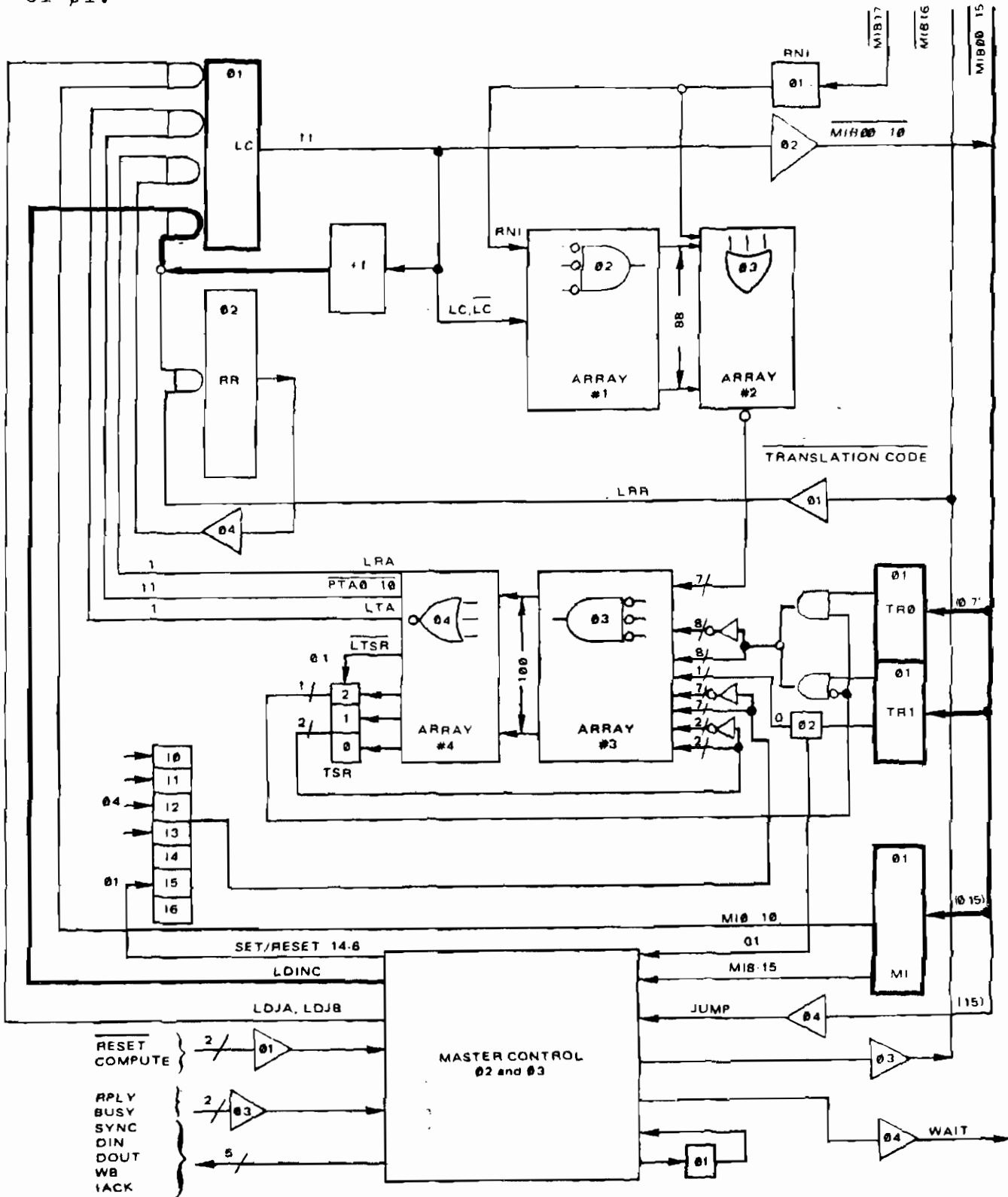
Figure 4-37. \emptyset 1 Data Flow
