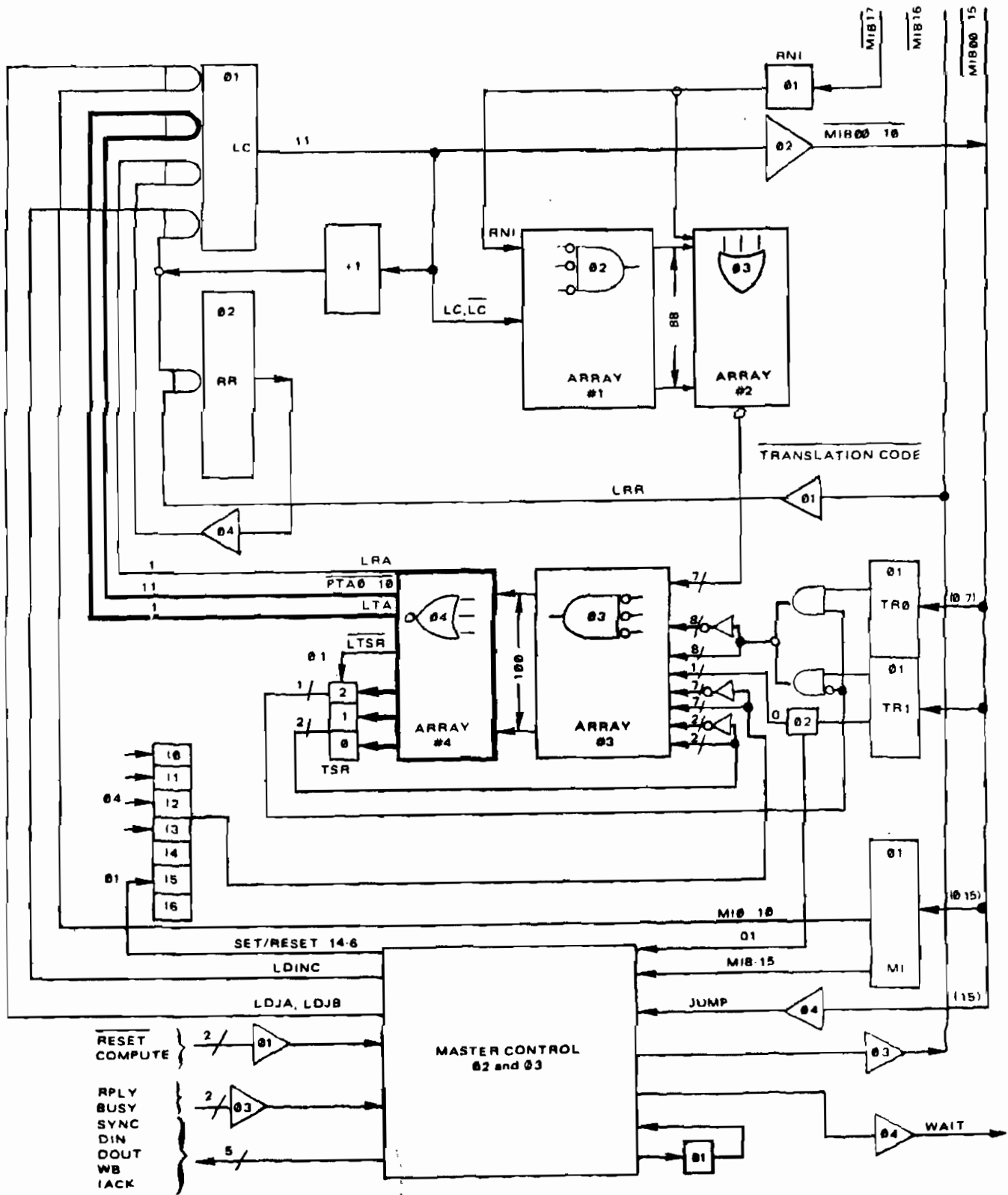
Figure 4-40. 04 Data Flow
