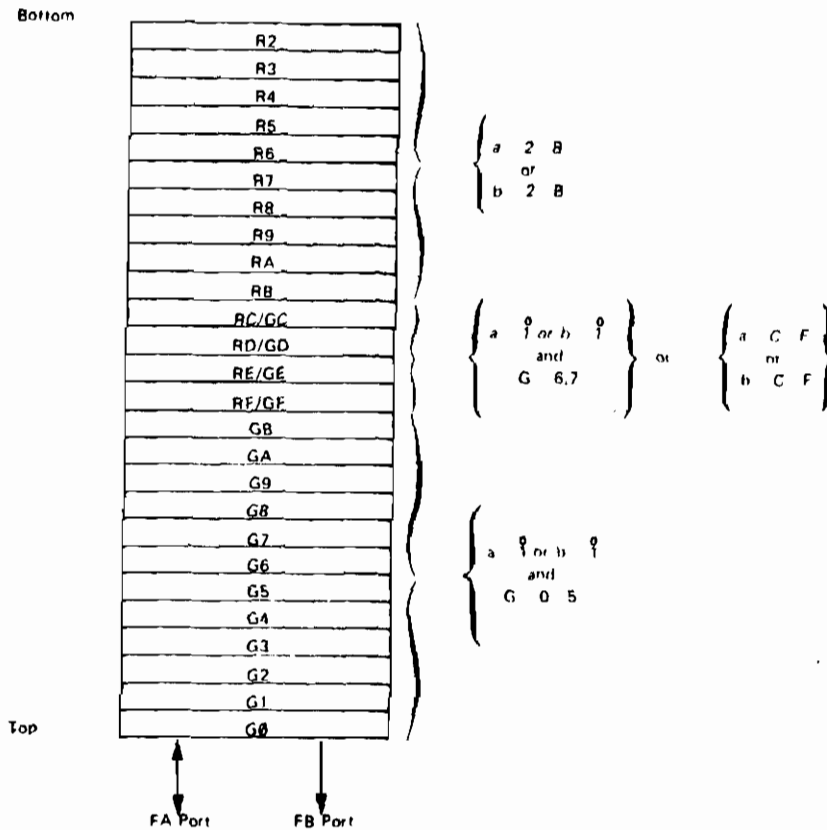
Figure 4-19. Register File
